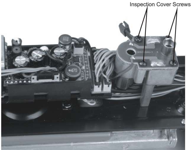
Inspecting the Smoke Unit Wick
