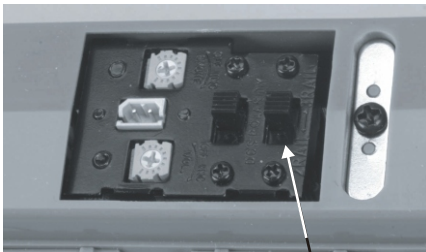
2-Rail/3-Rail Switch
