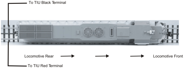
Proper 2-Rail Polarity wiring and locomotive orientation
