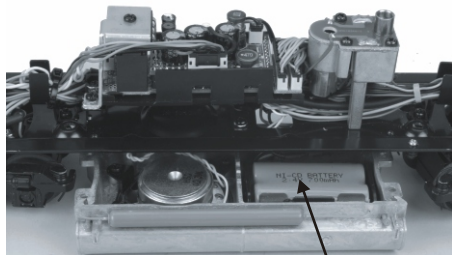
Lift Out Battery
